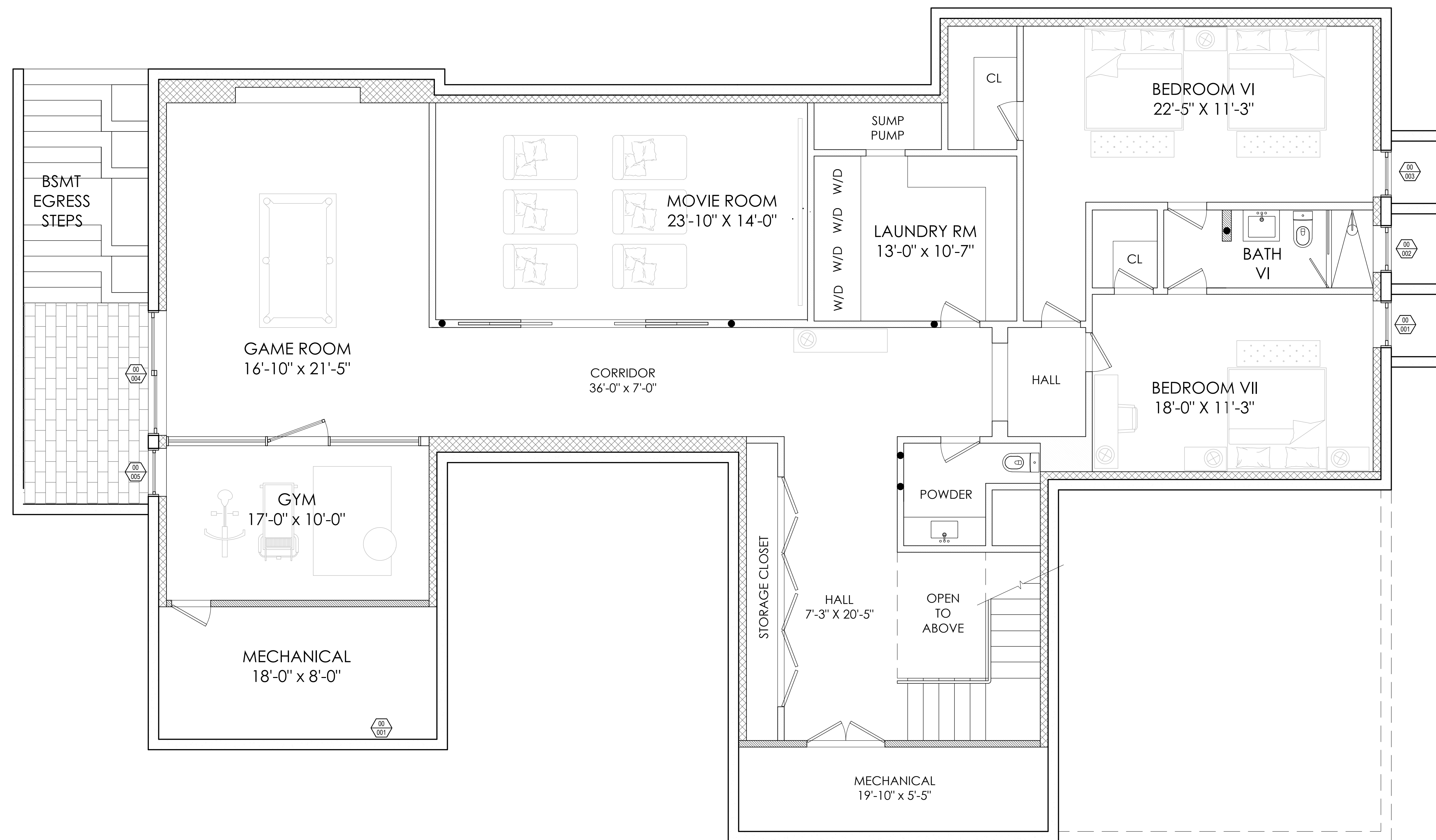
BASEMENT LEVEL
