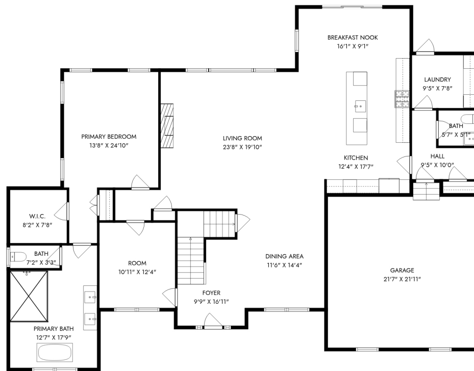
1ST FLOOR
