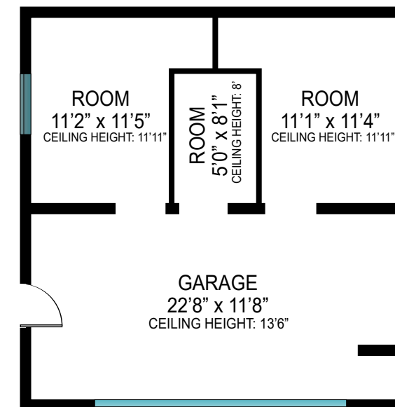
DETACHED GARAGE
